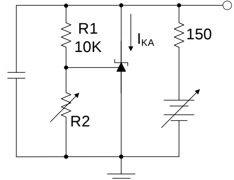
Test Circuit 4 for Z_{KA}
