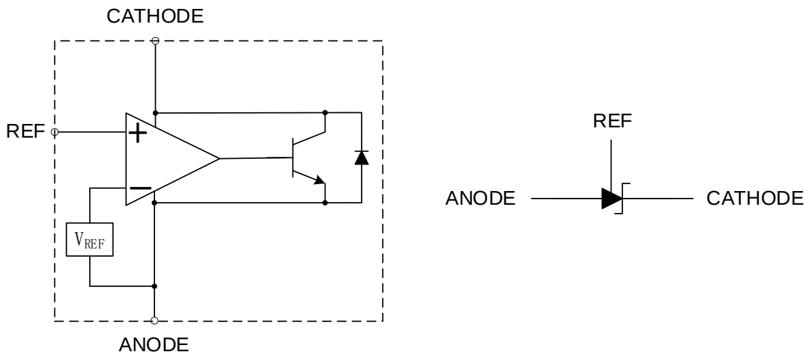
Figure 1 functional block diagram and symbol
