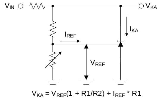
Test Circuit 2 for V_{KA} > V_{REF}
